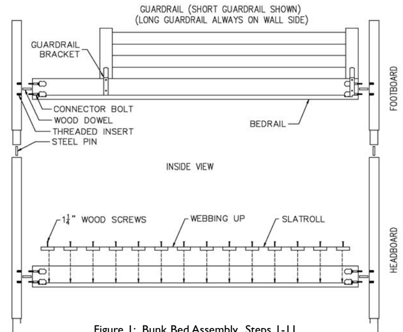
Figure 1: Bunk Bed Assembly Steps 1-11
