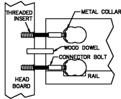
Figure 2: Bedrail Attachment
