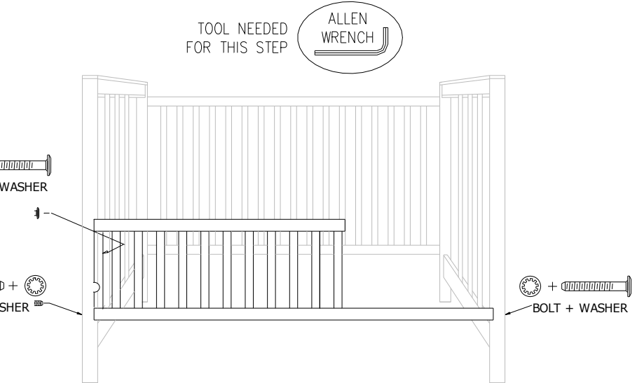
Toddler Rail (sold separately) (Mattress support spring should be in lowest position; it has been removed from this drawing for clarity.)
