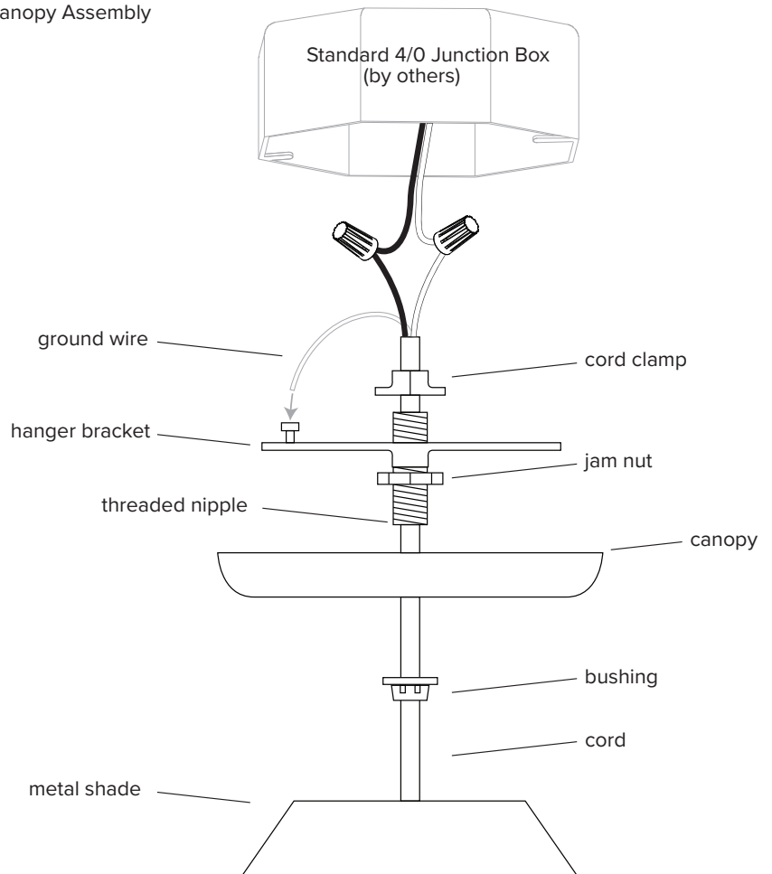
Canopy Assembly
