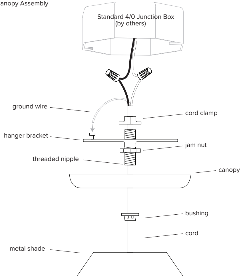
Canopy Assembly
