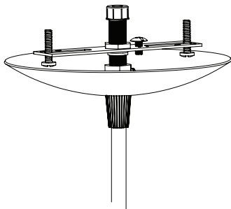
B. - Canopy assembly
