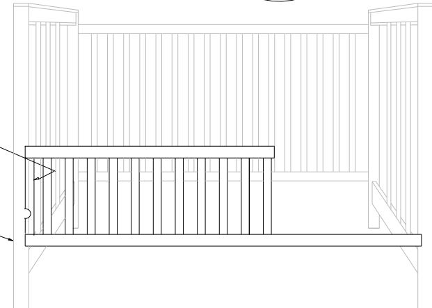
Toddler Rail (sold separately) (Mattress support spring should be in lowest position; it has been removed from this drawing for clarity.)
