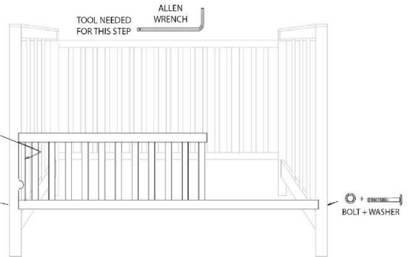
Toddler Rail (sold separately) (Mattress support spring should be in lowest position; it has been removed from this drawing for clarity.)
