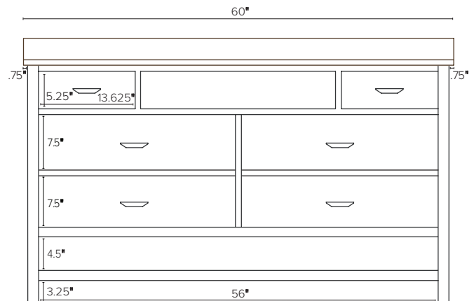
60w 21.75d 34h Single-Sink Vanity Tops with an overhang left side only or right side only are 59.25" wide.
