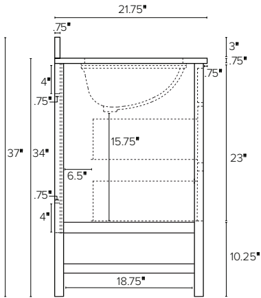
Side view measurements apply to all vanity sizes and both sink shapes.
