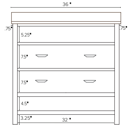
36w 21.75d 34h Single-Sink Vanity Tops with an overhang left side only or right side only are 35.25" wide.
