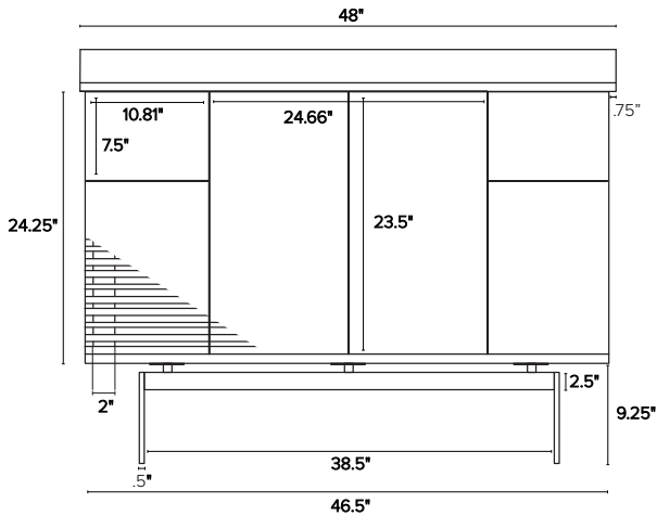
48w 21.75d 34h Single-Sink Vanity Tops with an overhang left side only or right side only are 47.25" wide.
