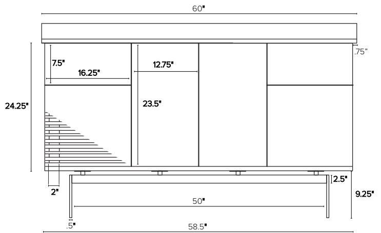
60w 21.75d 34h Single-Sink Vanity Tops with an overhang left side only or right side only are 59.25" wide.
