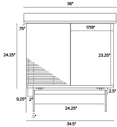
36w 21.75d 34h Single-Sink Vanity Tops with an overhang left side only or right side only are 35.25" wide.
