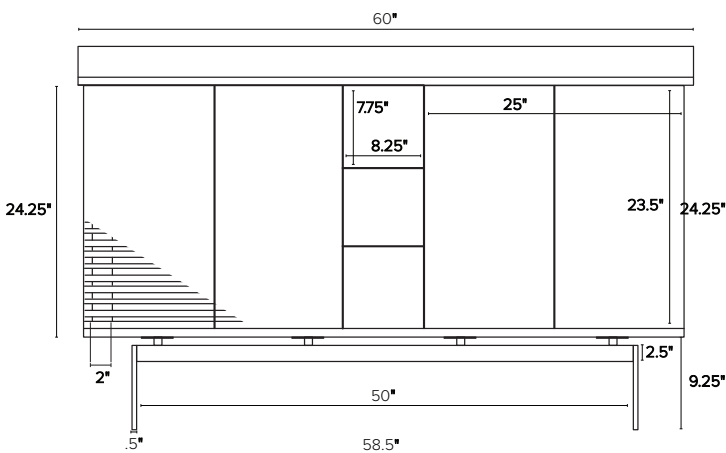
60w 21.75d 34h Double-Sink Vanity Tops with an overhang left side only or right side only are 59.25" wide.
