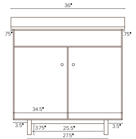
36w 21.75d 34h Single-Sink Vanity Tops with an overhang left side only or right side only are 35.25" wide.
