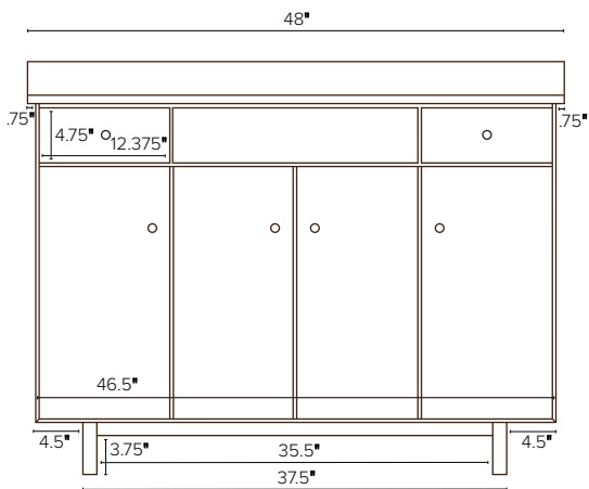
48w 21.75d 34h Single-Sink Vanity Tops with an overhang left side only or right side only are 47.25" wide.
