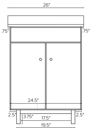
26w 21.75d 34h Single-Sink Vanity Tops with an overhang left side only or right side only are 25.25" wide.
