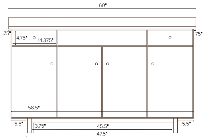
60w 21.75d 34h Single-Sink Vanity Tops with an overhang left side only or right side only are 59.25" wide.
