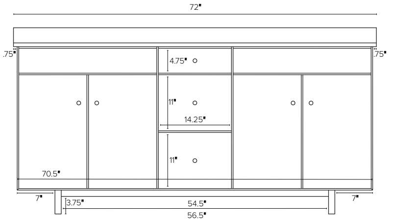
72w 21.75d 34h Double-Sink Vanity Tops with an overhang left side only or right side only are 71.25" wide.
