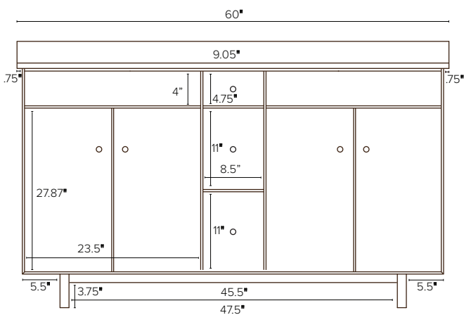
60w 21.75d 34h Double-Sink Vanity Tops with an overhang left side only or right side only are 59.25" wide.
