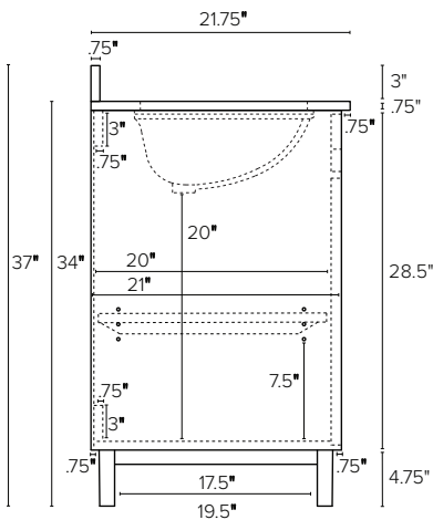
Side view measurements apply to all vanity sizes and both sink shapes.
